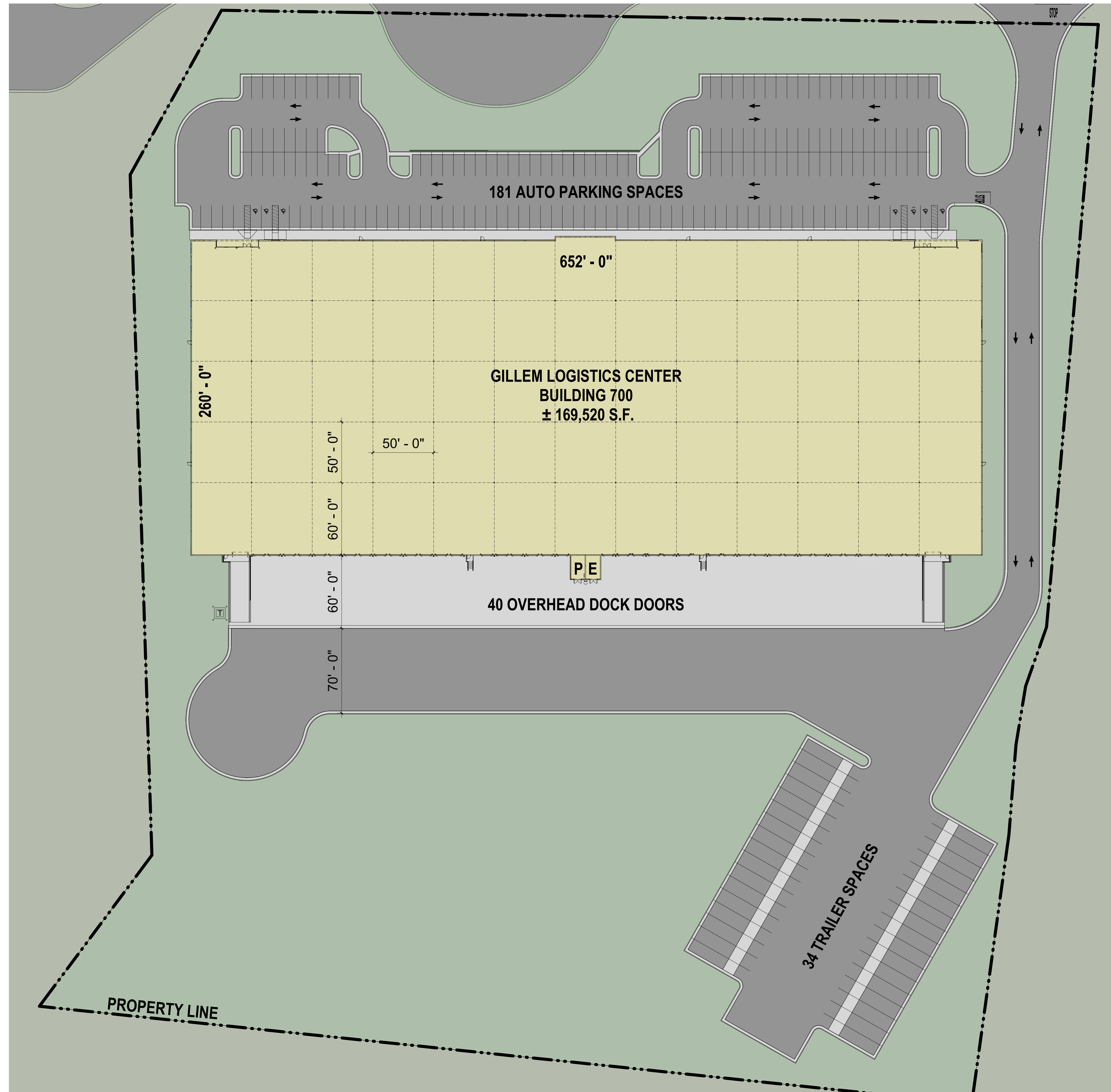
1 SK-01 ARCHITECTURAL SITE PLAN_COLORED 1" = 40'-0"
