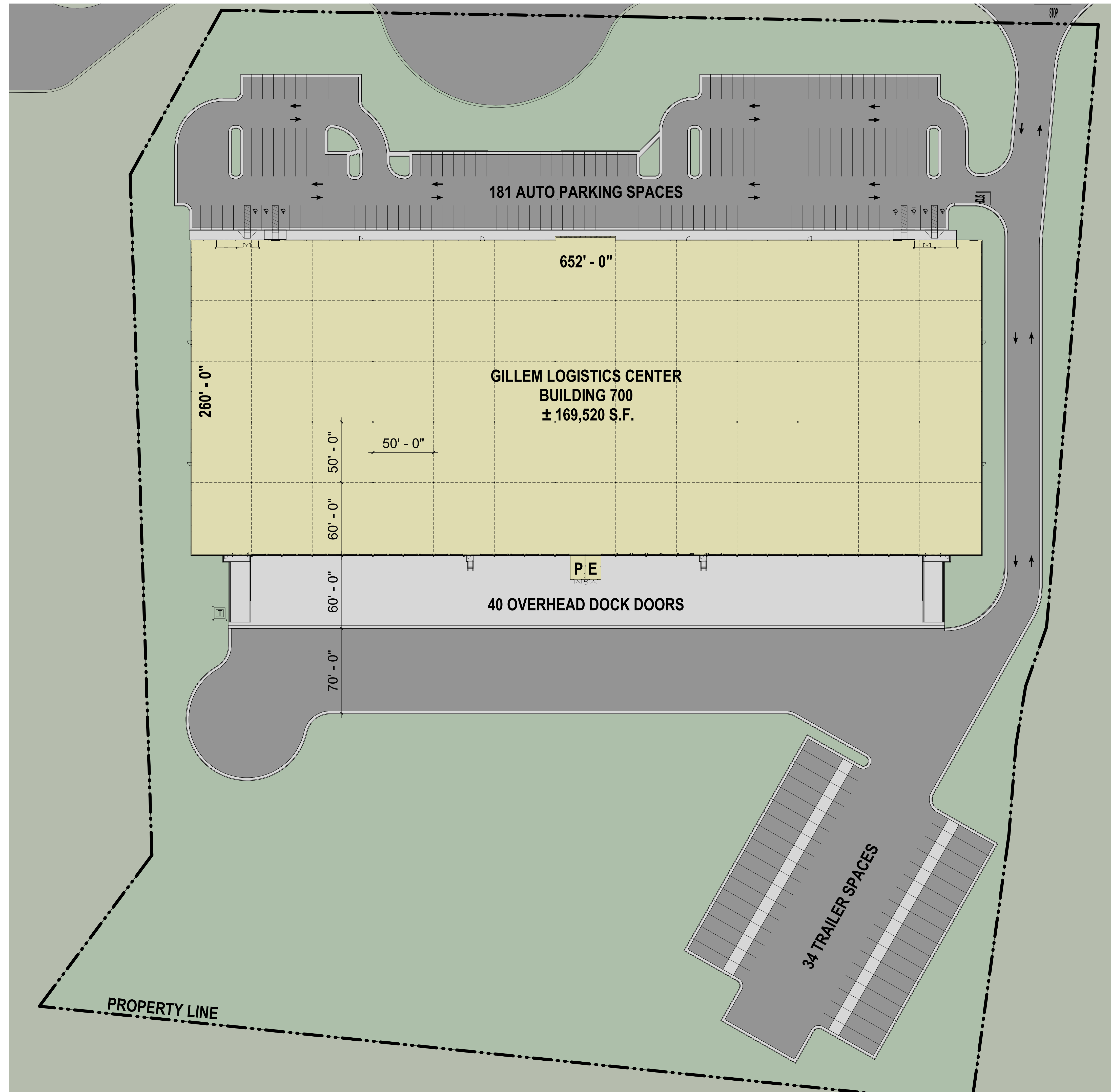
1 ARCHITECTURAL SITE PLAN_COLORED SK-01 1" = 40'-0"
